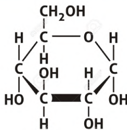
GLUCOSE MOLECULE
